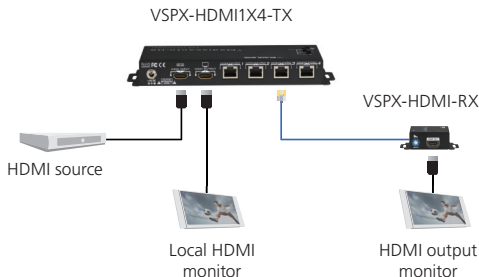
Figure 4-1. Connection diagram.
